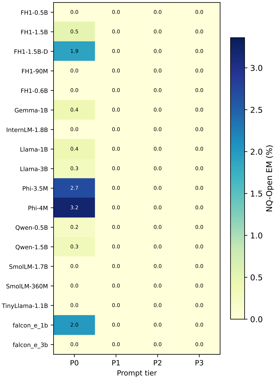
NQ-Open: Per-Model NQ-Open EM (%) (averaged over all edge settings)
