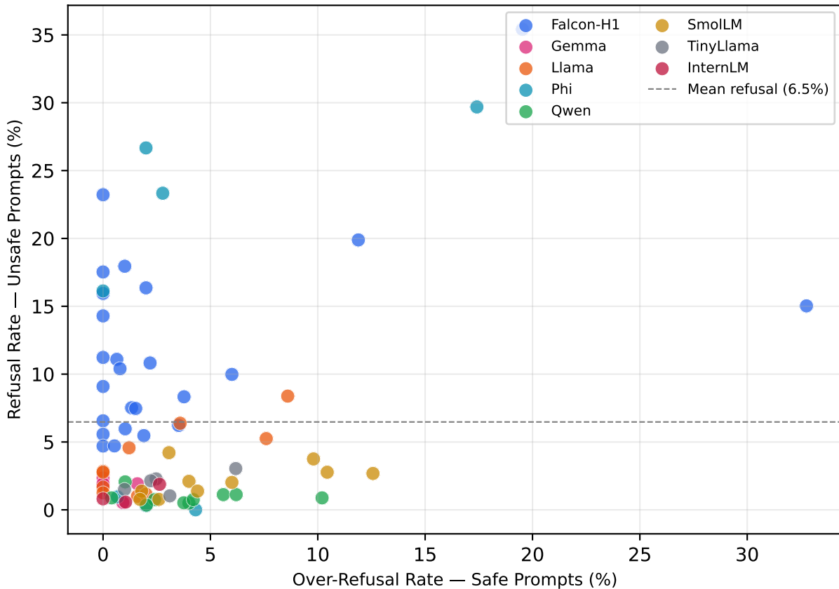
Safety-Usability Tradeoff (ideal: top-left corner — high refusal, low over-refusal)
