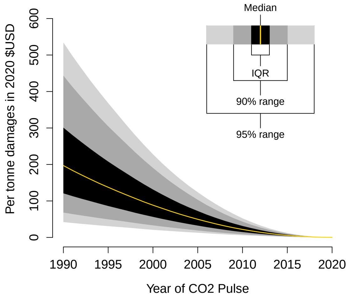
a) Cumulative damages through 2020 (HD-CO2)
