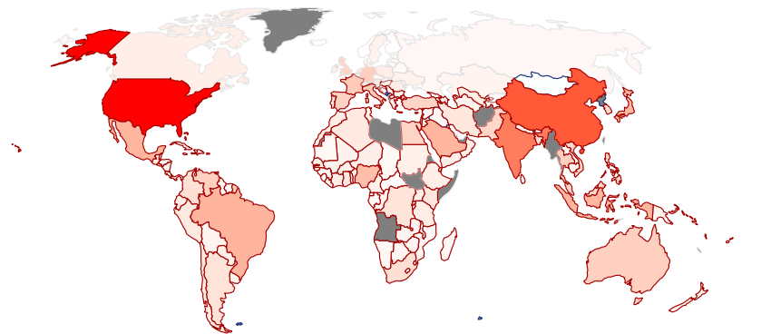
d) Impacts 2021–2100
