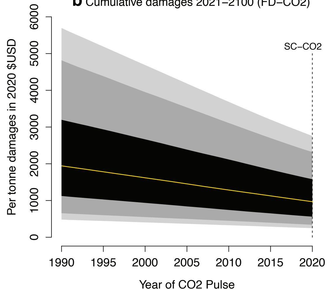
b Cumulative damages 2021–2100 (FD-CO2)
