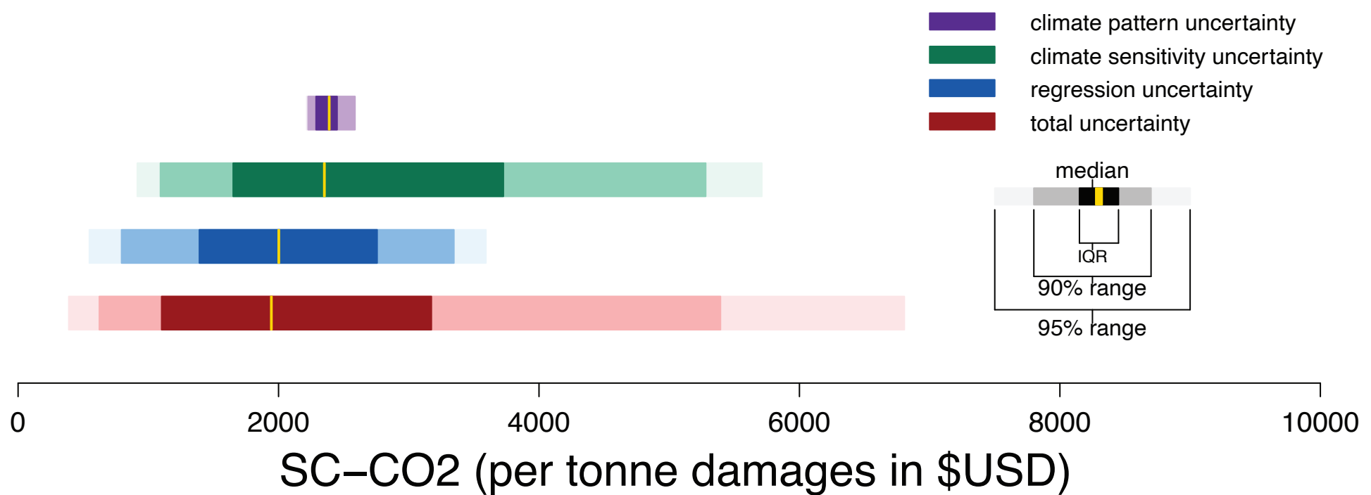
c Sources of uncertainty in SC-CO2 Estimation
