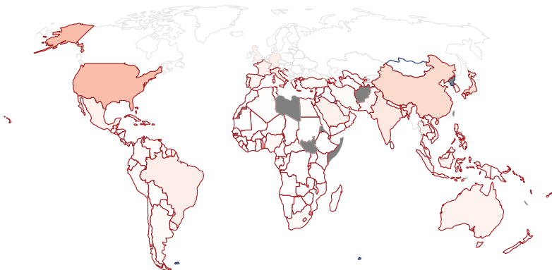
a Impacts through 2020 of 1t pulse in 1990
