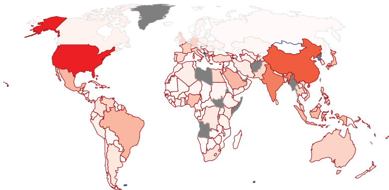
b Impacts 2021–2100 of 1t pulse in 1990
