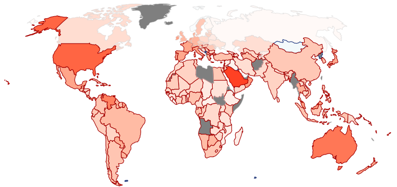
d Impacts per capita 2021–2100 of 1t pulse in 1990
