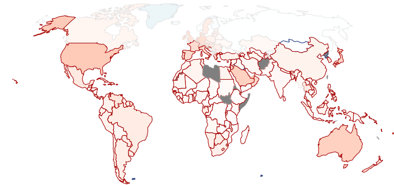
c Impacts per capita through 2020 of 1t pulse in 1990
