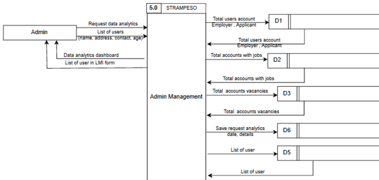
Figure 17: Level 0 of Proposed System, Process 5.0
