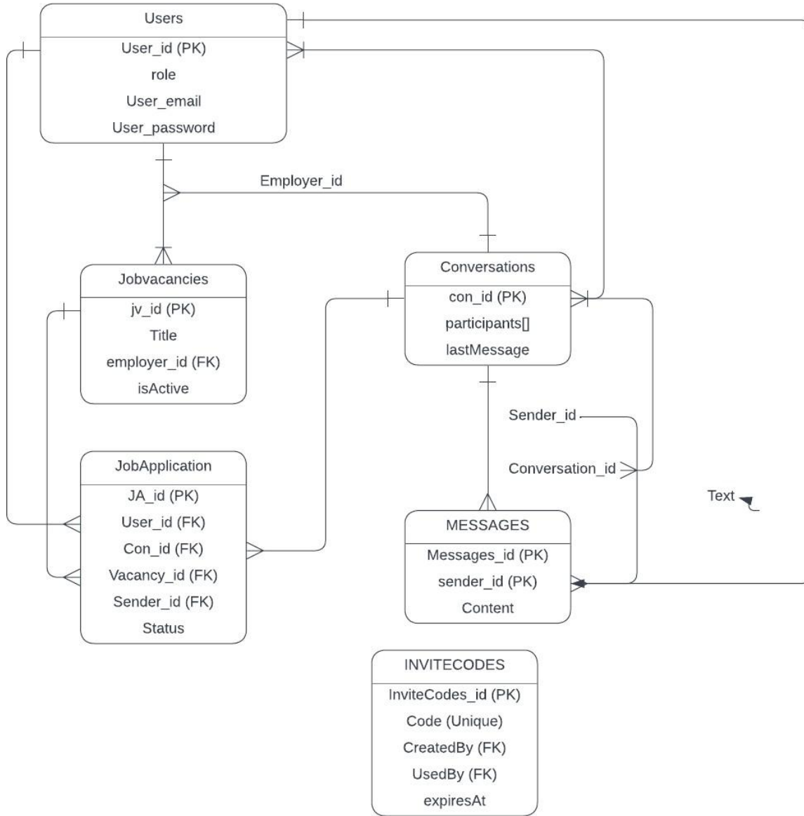
Figure 2: Database Schema
