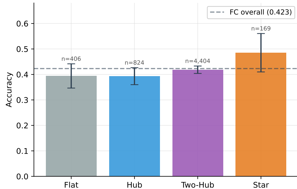
GPQA
