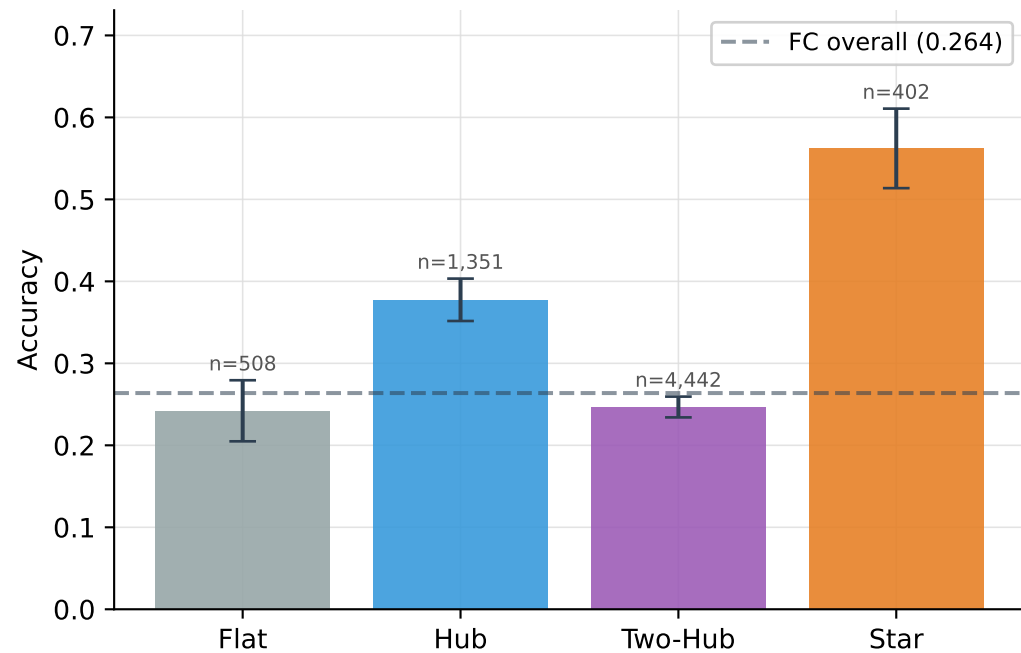
HiddenBench
