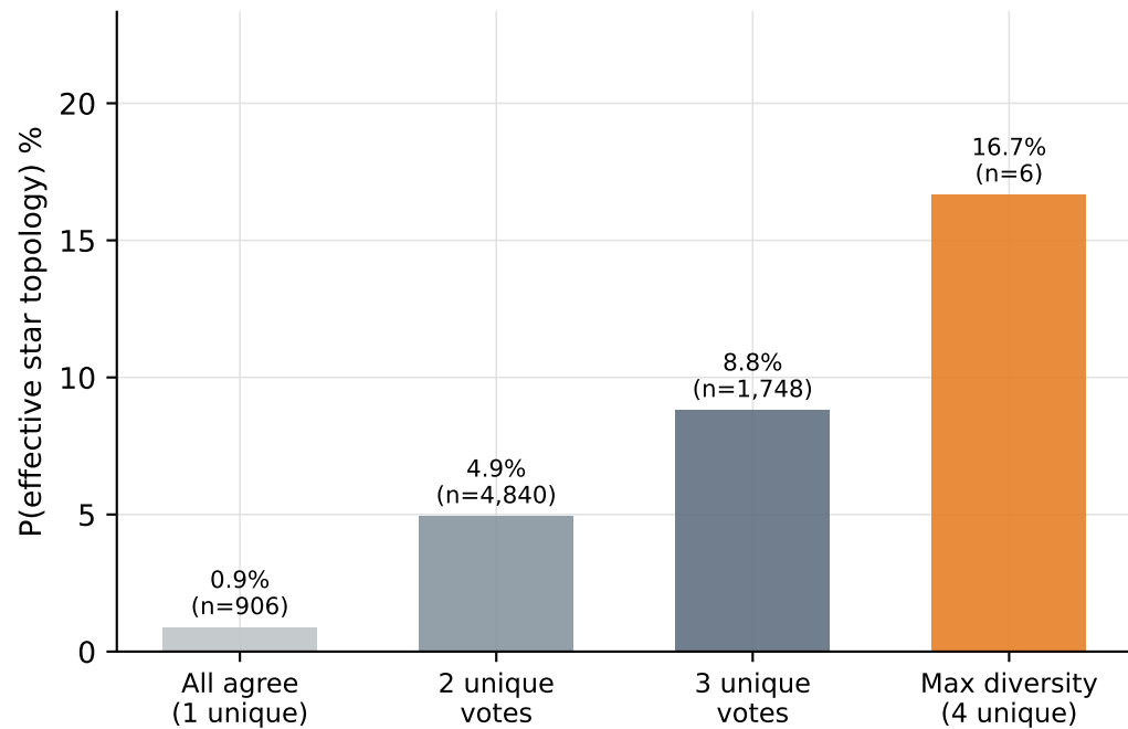
HiddenBench
