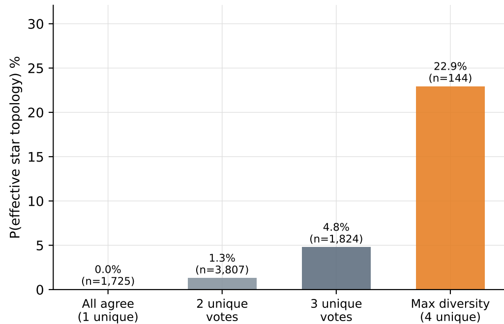
GPQA
