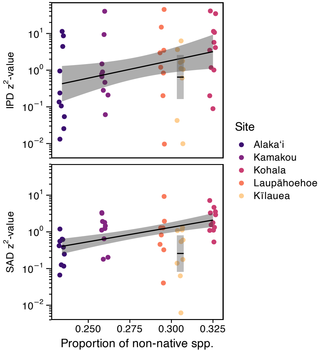
Supplementary Figure S5: Relationship between proportion of non-native species and deviation from METE. Kīlauea was excluded from the overall analysis to be able to compare it separately to the overall trend. Gray regions represent 95% confidence envelopes (or confidence interval for Kīlauea) and solid lines are expected values.
