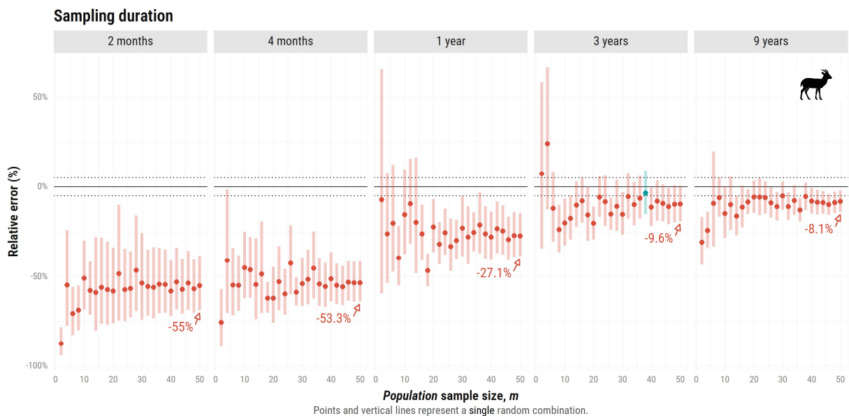
24 25 Figure S3.2. Relative error (%) in home range estimates (AKDE) as a function of population sample size ( m ), ranging from 2 to 50 simulated Mongolian 26 gazelles ( Procapra gutturosa ). Each vertical facet corresponds to one of five sampling durations: 2 months, 4 months, 1 year, 3 years, and 9 years. The 27 plot shows mean estimates based on a single combination of individuals per m (no resampling); estimates in blue are within the error threshold and 28 in red if estimates fall outside of it. Horizontal dotted lines mark the \pm 5\% error threshold.
