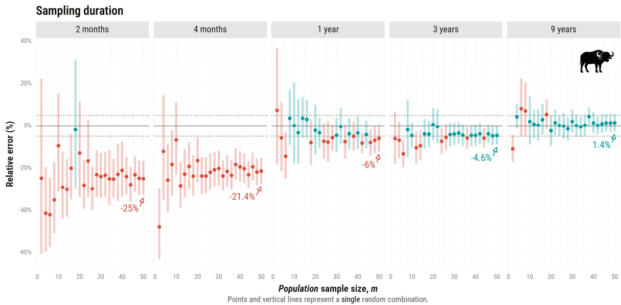
19 20 Figure S3.1. Relative error (%) in home range estimates (AKDE) as a function of population sample size ( m ), ranging from 2 to 50 simulated African 21 buffalos ( Syncerus caffer ). Each vertical facet corresponds to one of five sampling durations: 2 months, 4 months, 1 year, 3 years, and 9 years. The 22 plot shows mean estimates based on a single combination of individuals per m (no resampling); estimates in blue are within the error threshold and 23 in red if estimates fall outside of it. Horizontal dotted lines mark the \pm 5\% error threshold.
