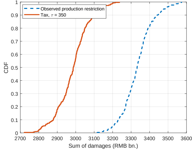
Figure Response.1: Total Damage CDFs: Production Restriction and Optimal Tax
