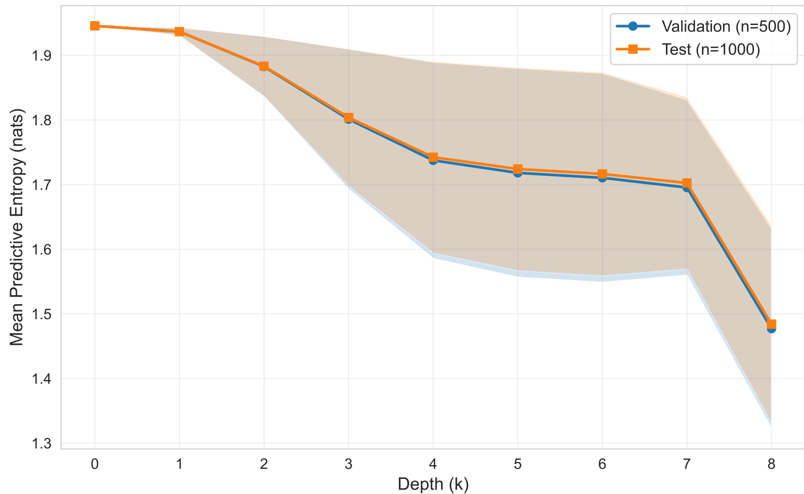
Predictive Entropy vs Depth ( \pm 1 std, n_seeds=3) Cora - GCN
