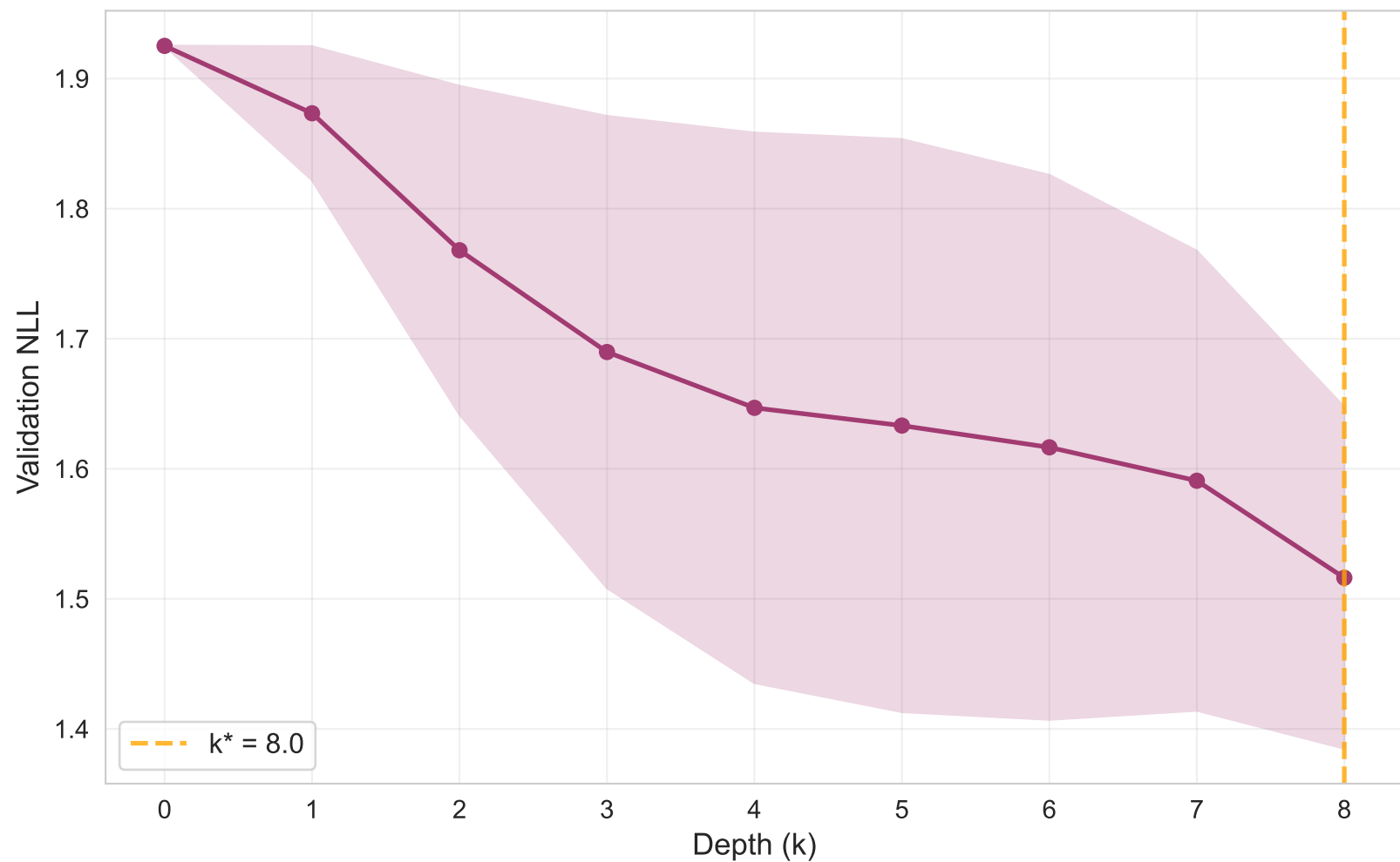
Validation NLL vs Depth ( \pm 1 std, n_seeds=3) Cora - GCN
