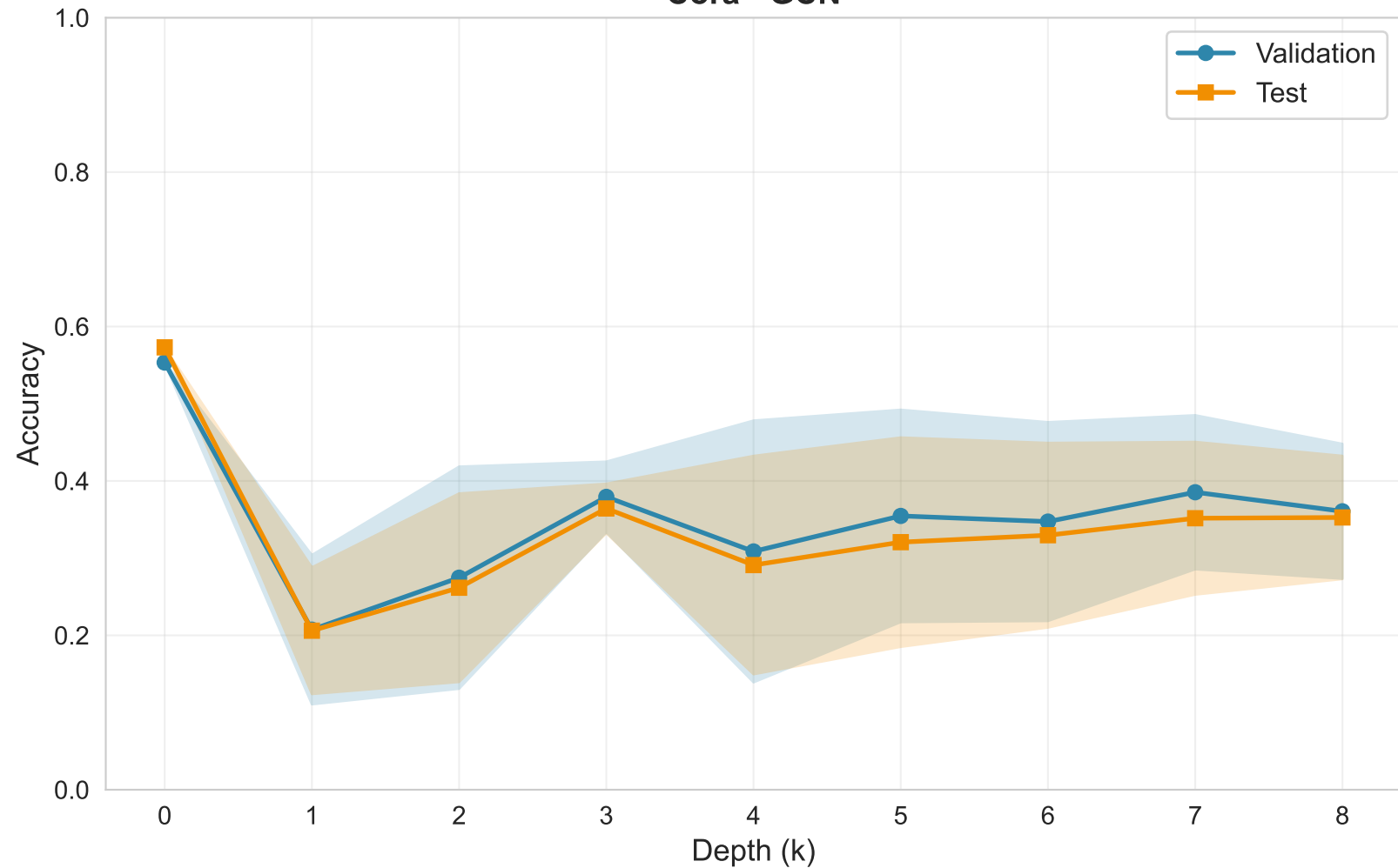
Accuracy vs Depth ( \pm 1 std, n_seeds=3) Cora - GCN
