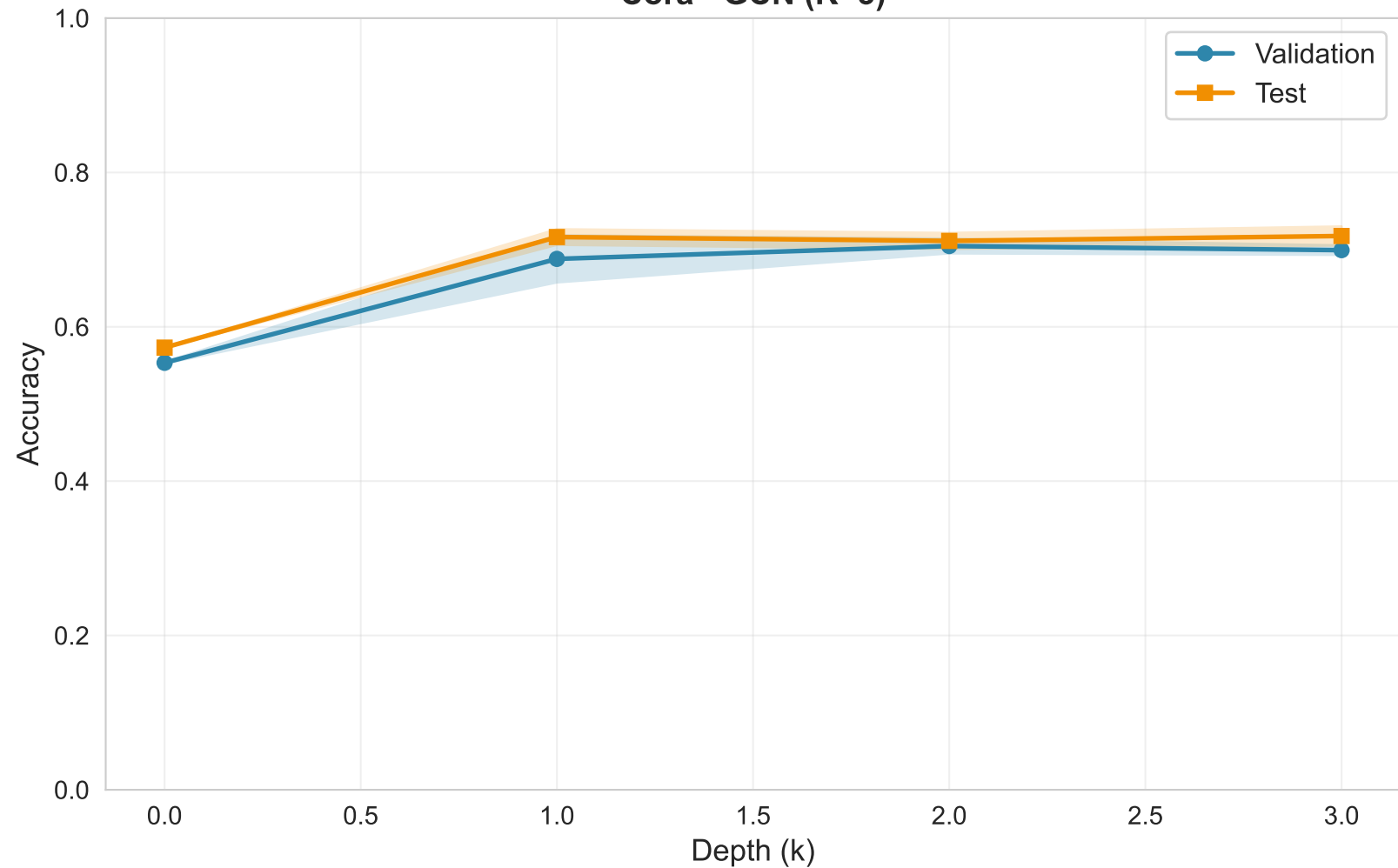
Accuracy vs Depth ( \pm 1 std, n_seeds=3) Cora - GCN (K=3)
