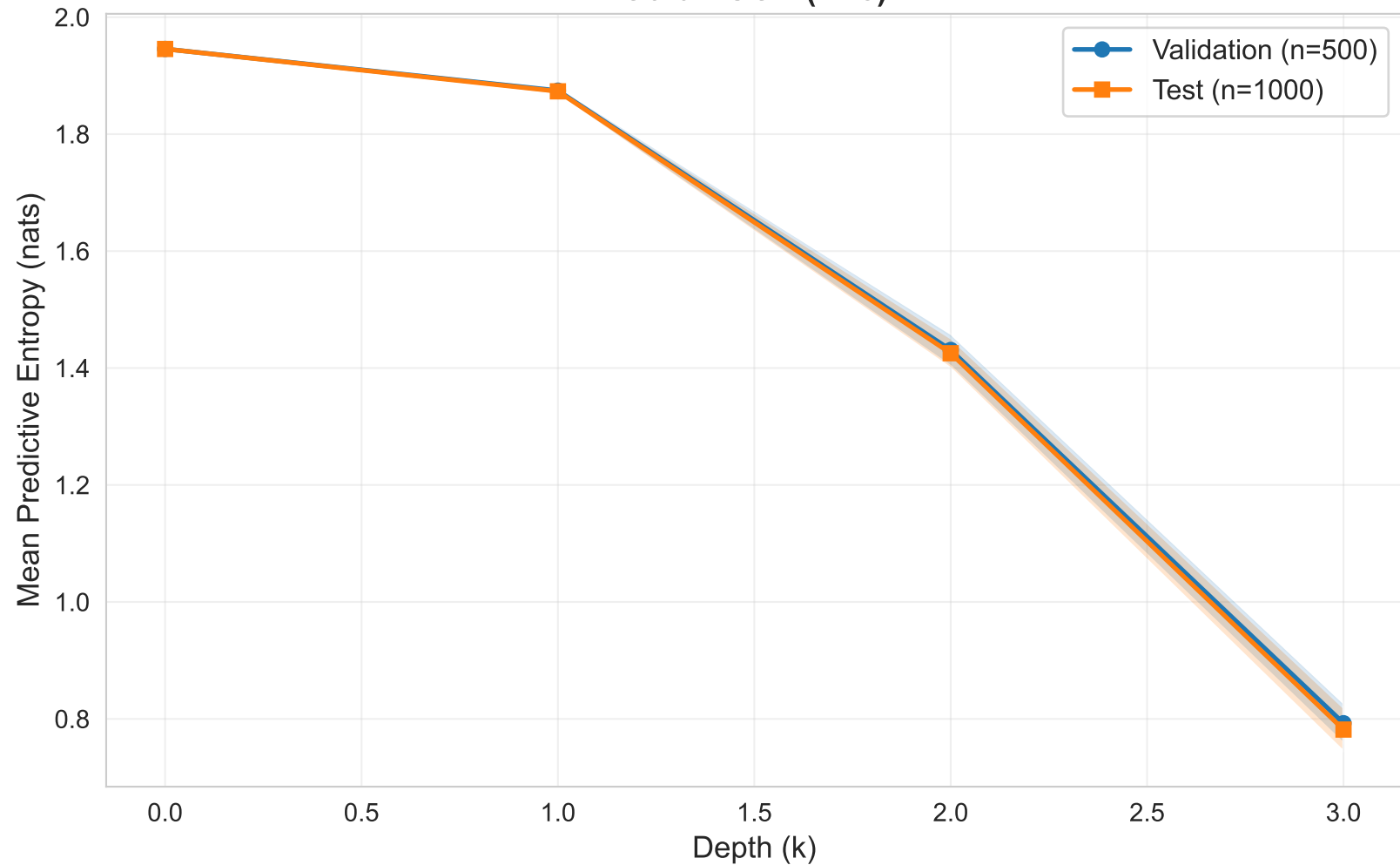
Predictive Entropy vs Depth ( \pm 1 std, n_seeds=3) Cora - GCN (K=3)
