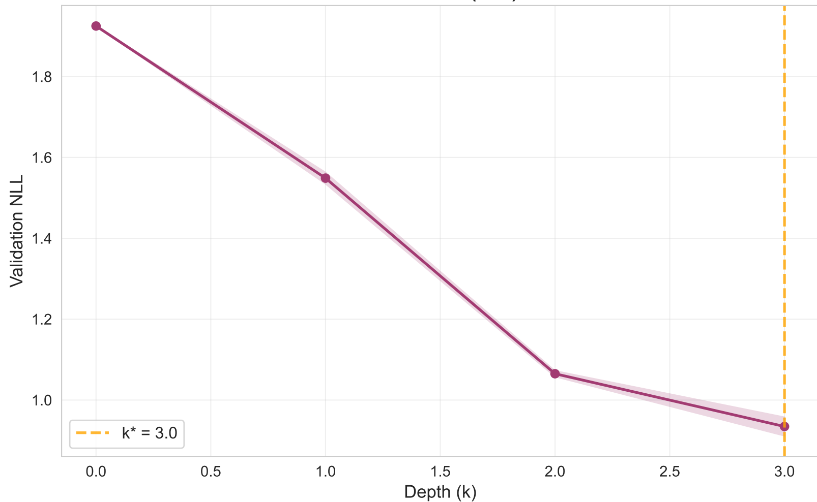
Validation NLL vs Depth ( \pm 1 std, n_seeds=3) Cora - GCN (K=3)
