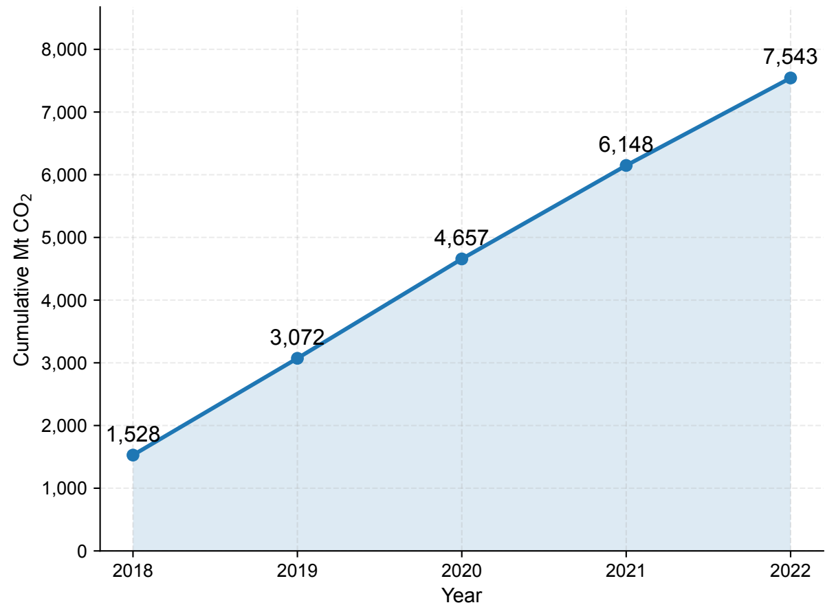
B. Cumulative livestock-related LUC emissions
