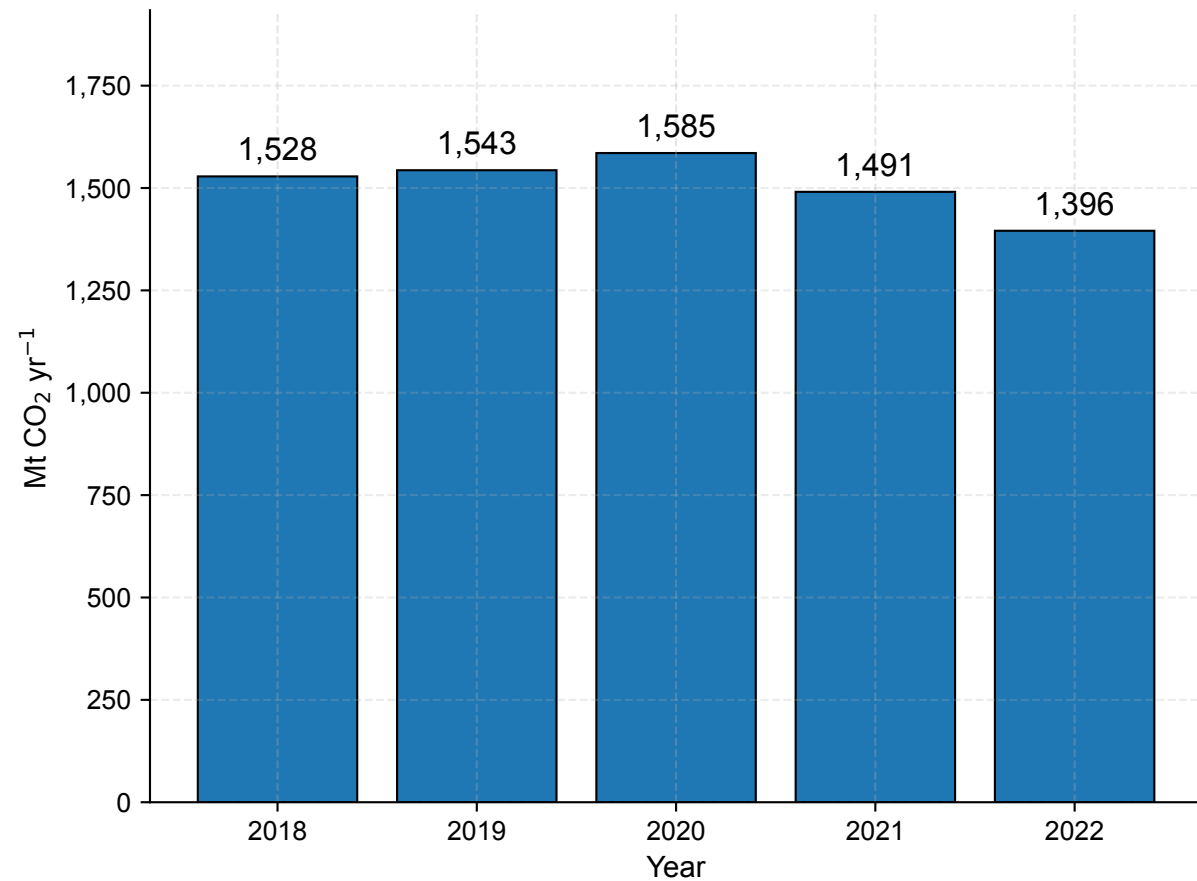
A. Annual livestock-related LUC emissions
