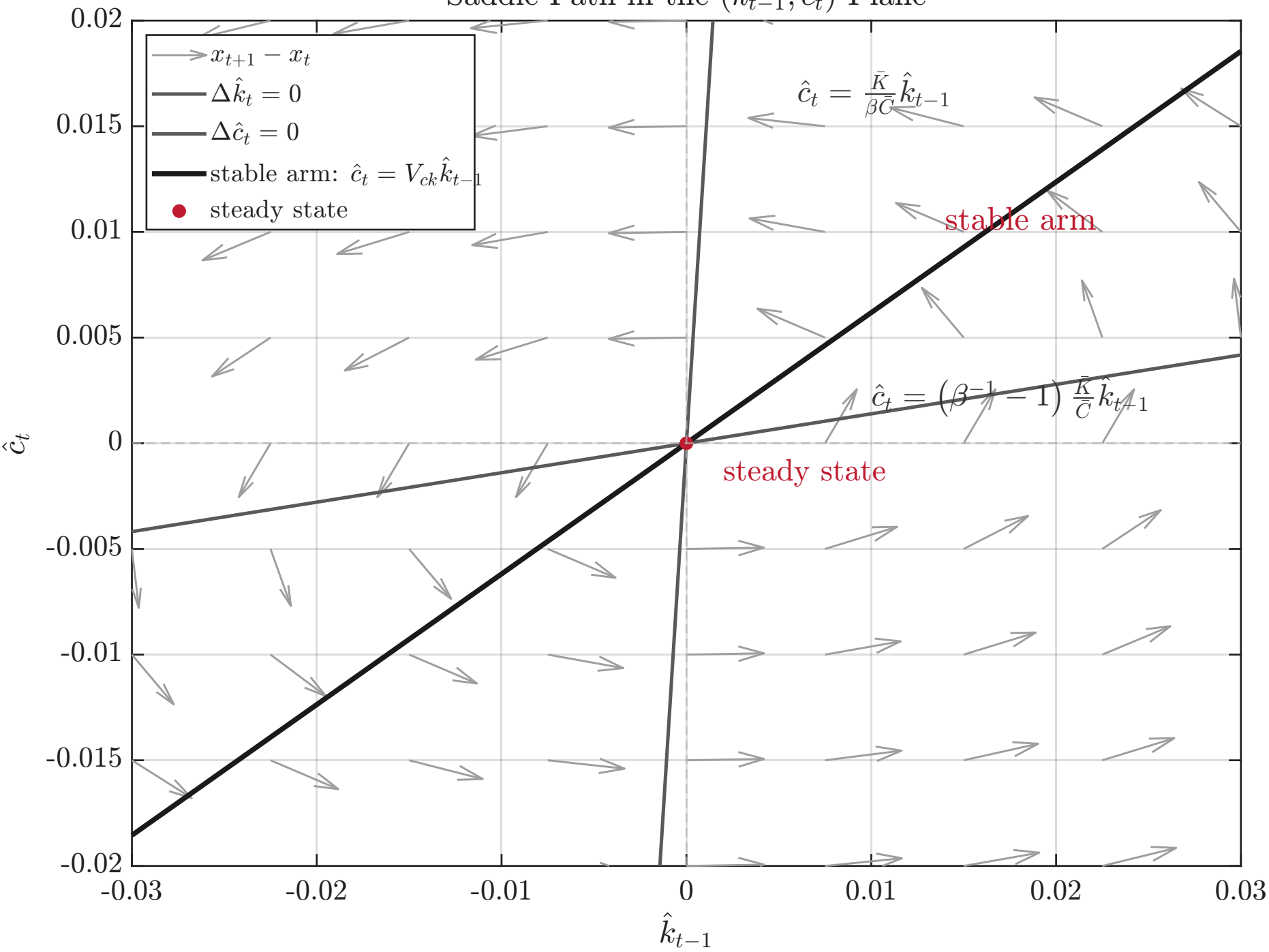
Saddle Path in the (\hat{k}_{t-1}, \hat{c}_t) Plane
