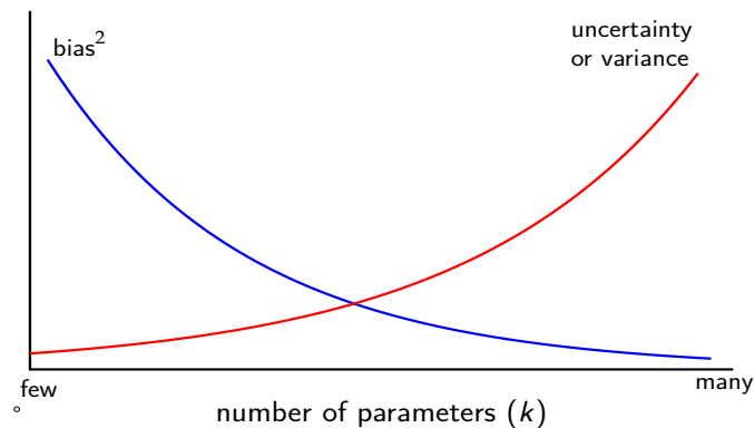
Figure 4.1: Fundamental relationship between the number of parameters in a model ( k ), and the square of the bias (related to overall model fit to the data), and parameter uncertainty (precision of parameter estimates).
