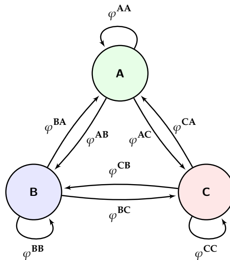
Figure 10.1: Schematic representing a typical multi-state model. Here, there are 3 states (A, B and C), with the arrows indicating directional movement between states over a given time interval. The probability of moving, conditional on surviving, from state i \rightarrow j over the time interval is specified by parameter \varphi^{ij}
