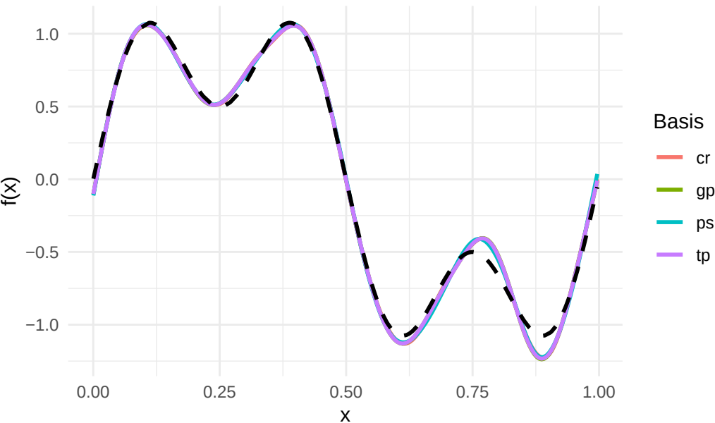
Smooth estimates by basis type
