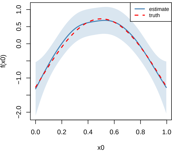
s(x_0)
