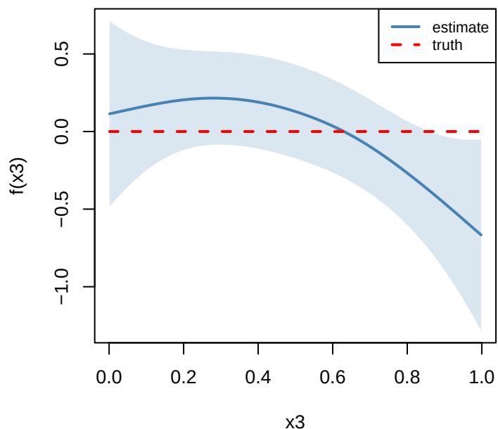
s(x_3)
