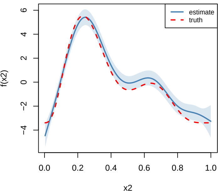
s(x_2)
