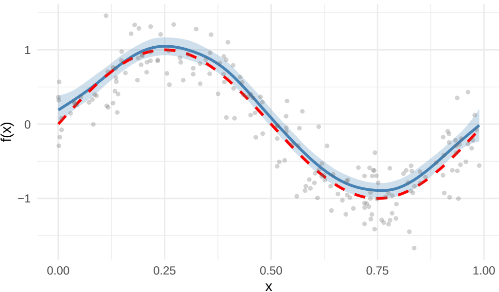
Estimated smooth with confidence band
