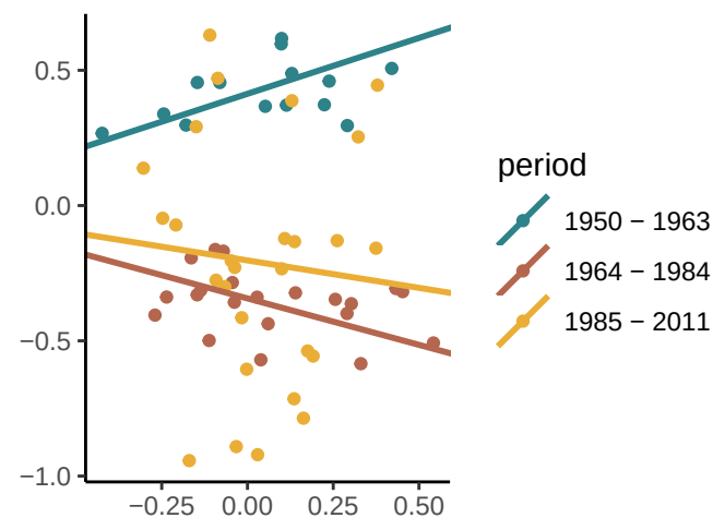
E. Time-Varying Slope & Intercept
