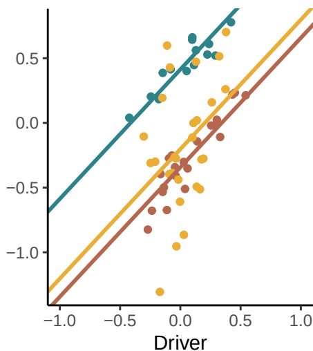
D. Time-Varying Intercept
