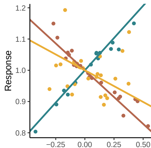
C. Time-Varying Slope
