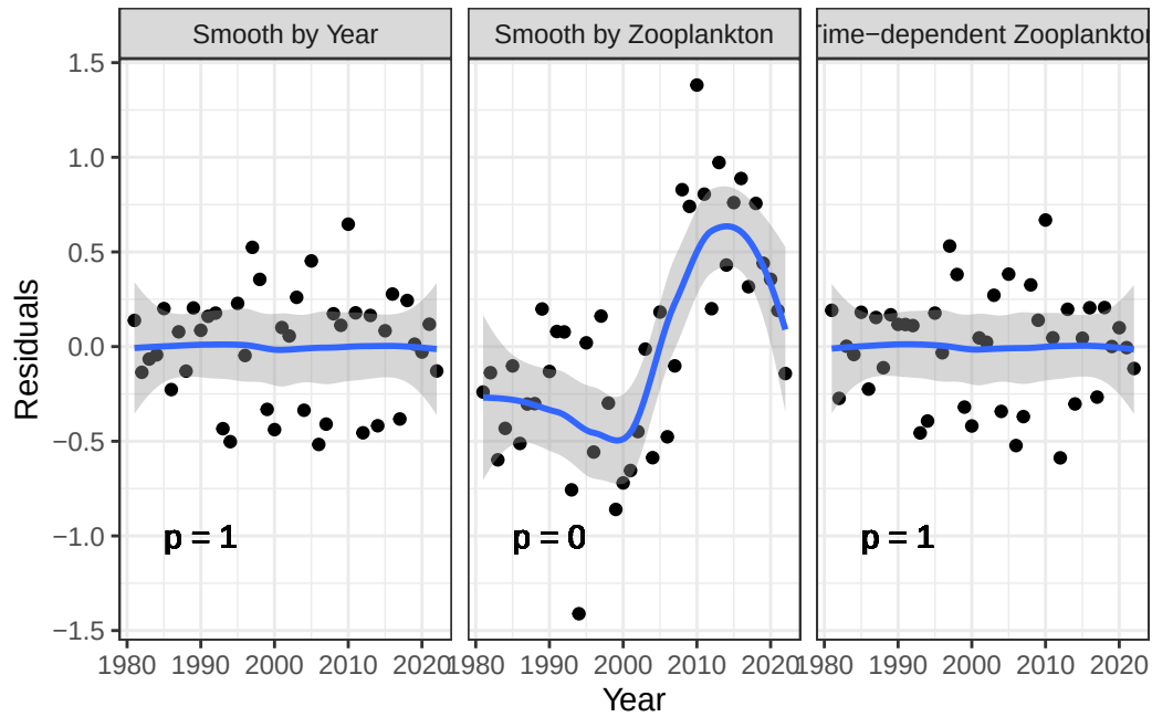
Figure S1.6: Model residuals for a smooth on zooplankton abundance, a smooth on year, and a smooth on year by zooplankton. p-value denotes the significance of the trend in residuals through time.
