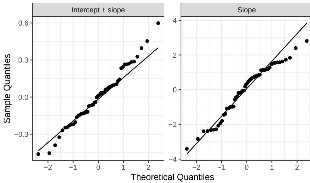
GAM Residuals
