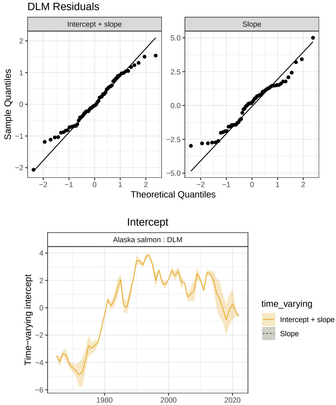
Figure S7: Time-varying intercept of the DLM model representing the relationship between SST anomalies and salmon catch.
