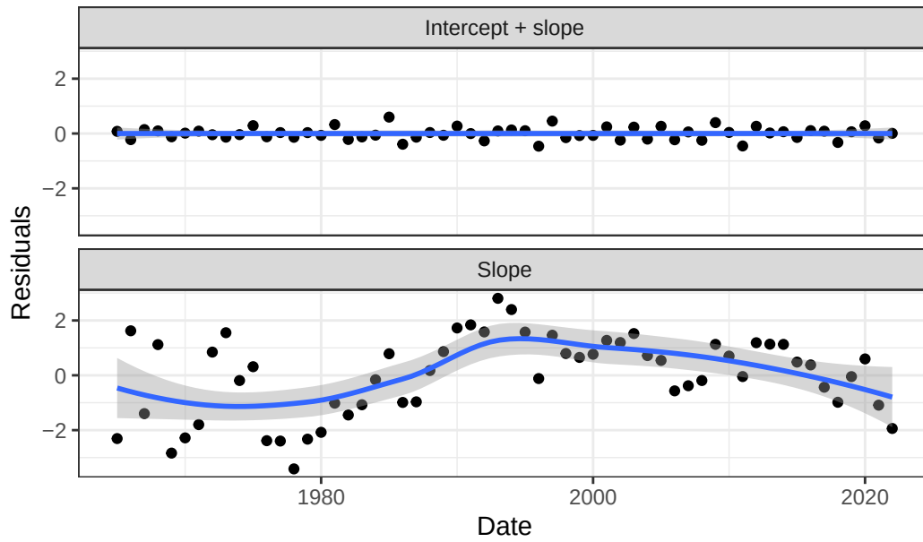
GAM Residuals
