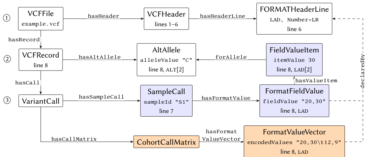
Figure 1: Selected resources for the first record (line 8) of Listing 1, walked through in steps ①–③. Purple nodes are expanded -profile resources, orange condensed . Depth 30 is associated with "C", the sample's local allele, not with ALT[1], "A". LAA has no node of its own because its resolution is already applied in forAllele . The two dashed links show that both profiles resolve to the same FieldDefinition . Lines 9–10, the expanded resources for S2, other fields, allele "A", and header lines are omitted; the condensed vector holds both samples, tab-separated.
