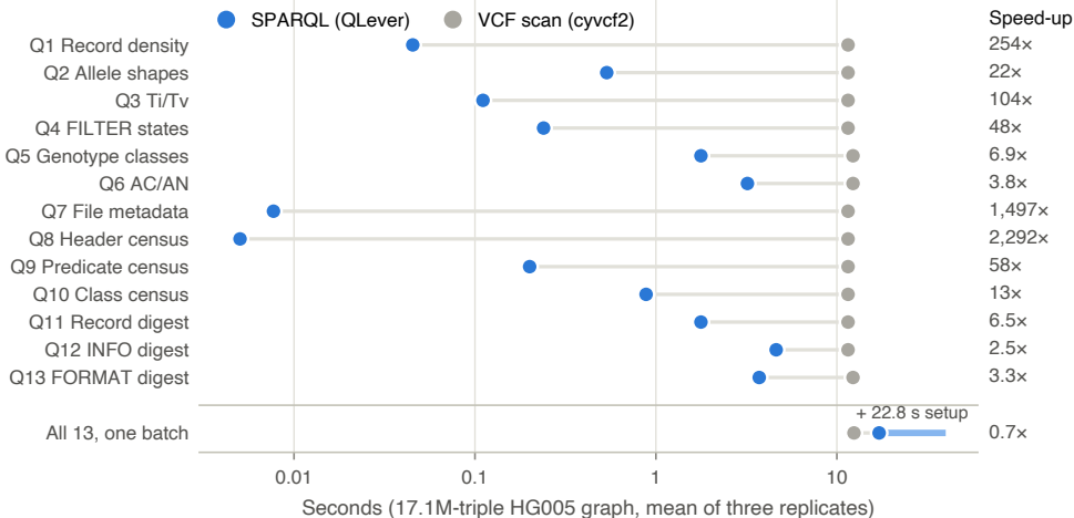
(a) Per question, SPARQL beats a VCF scan; for the whole batch, one scan wins
