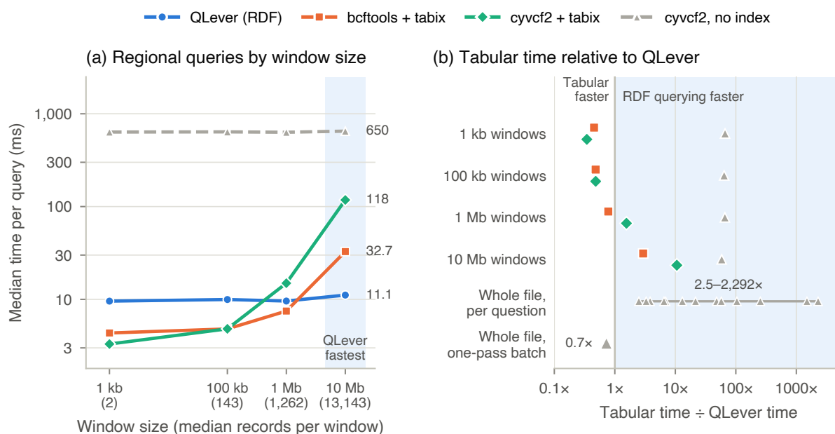
Figure 5. Where tabular parsing is and is not stronger than RDF querying (main Figure 8). (a) Median time per regional query on 100,000 HG005 records, by window size (median records per window in parentheses). (b) Every comparison as tabular time divided by QLever time; points in the shaded region are those where tabular parsing was slower. Setup is excluded: 23.2 s for QLever's index against 0.48 s for bgzip and tabix.
