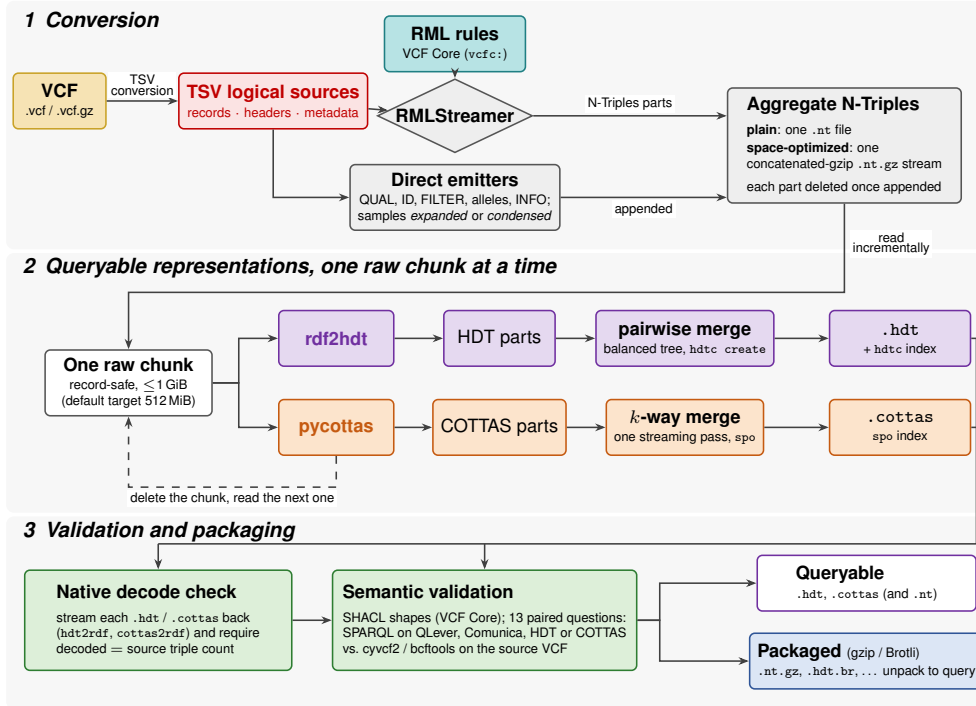
Fig. 1 VCF-RDFizer v3.1.0 pipeline. (1) Conversion: the VCF is split into three TSV logical sources; RMLStreamer applies the RML rules to emit VCF Core N-Triples, and direct emitters add the row-dependent fields RML cannot type per row (QUAL, ID, FILTER, alleles, structured INFO) and the samples in the expanded or condensed profile. Every part is appended to one aggregate and then deleted: a plain .nt file, or in space-optimized mode a concatenated-gzip .nt.gz stream. (2) Queryable representations: the aggregate is read incrementally and only one record-safe raw chunk exists at a time; rdf2hdt and pycottas each consume it before it is deleted. HDT parts are merged pairwise in a balanced tree with hdtc and indexed; COTTAS parts are merged in one streaming k -way pass with an spo index. (3) Validation and packaging: each artifact is decoded back and its triple count compared with the source; the graph is then checked against the VCF Core SHACL shapes and against thirteen questions answered both by SPARQL and by a VCF parser. HDT and COTTAS files are queryable as written; gzip or Brotli packages are for transport and must be unpacked before querying.
