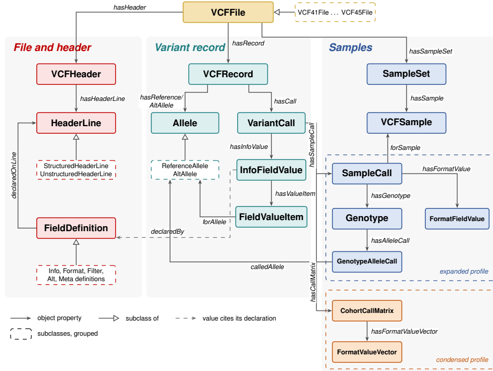
Fig. 2 VCF Core Vocabulary, simplified class diagram. The backbone of the model VCF-RDFizer v3.1.0 emits, drawn from the ontology bundle it ships; all class and property names carry the vcf: prefix, https://w3id.org/vcf-core/vocab# . A VCFFile , typed with its version-specific subclass, links to three layers. In the header layer, header lines carry the INFO, FORMAT, FILTER, ALT and META definitions that values cite through declaredBy . In the record layer, each VCFRecord has ordered alleles and a VariantCall carrying the INFO values, whose Number=A/R/G items point at the allele they describe. In the sample layer, the call links either to per-sample SampleCalls , genotypes and allele calls ( expanded profile ) or to one CohortCallMatrix of sample-ordered vectors ( condensed profile ). Structural-variant, phasing, local-allele and value-typing classes are omitted; the full vocabulary, with worked examples, is documented at https://ecrum19.github.io/vcf-core-vocabulary/ .
