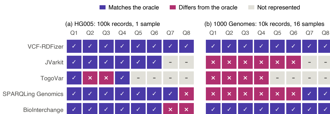
Figure 7. Only VCF-RDFizer's graphs answered every content question as the oracle did on both shared inputs (main Figure 5). Each cell is one of the content questions Q1–Q8, ported to the converter's vocabulary and answered from its graph: ✓ as the oracle, × differently, – not in the graph. Q1–Q4 summarize records, Q5–Q6 genotypes, and Q7–Q8 the header. (a) 100,000 HG005 records, one sample. (b) 10,000 records and 16 samples of the 1000 Genomes chromosome-20 call set. JVarkit merges records sharing CHROM, POS, and REF; TogoVar drops symbolic and * alleles and writes no samples or header; SPARQLing Genomics writes only carriers' calls (1,401 of 10,000 cohort records); BioInterchange's HG005 header document is invalid JSON.
