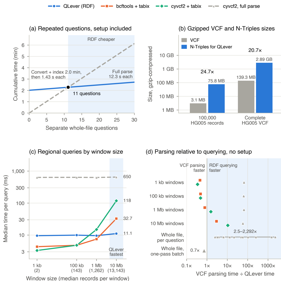
Figure 5. Where VCF parsing is and is not faster than RDF querying (main Figure 9). All panels use 100,000 HG005 records. (a) Repeated whole-file questions with setup included: a full cyvcf2 parse per question against 2.0 min, measured in a rerun, to convert the records to gzip-framed N-Triples and index them in QLever, breaking even at 11 questions. (b) Gzip-compressed sizes of the VCF and of the N-Triples QLever indexes, also for the complete HG005 VCF. (c) Median time per regional query by window size (median records per window in parentheses). (d) Every comparison as VCF parsing time divided by QLever time, setup excluded; points in the shaded region are those where VCF parsing was slower.
