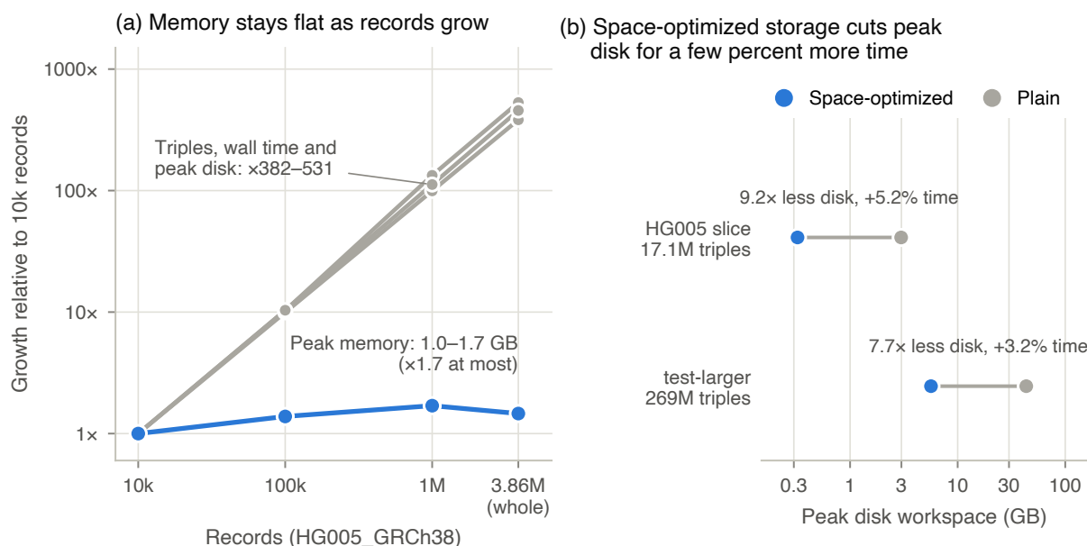
Figure S3. Record scaling and workspace. (a) Growth relative to 10,000 HG005 records, using medians of three replicates except the single whole-genome run. (b) Peak workspace and the end-to-end time cost of space-optimized storage on two inputs. Triple counts and final artifacts agree between storage modes; both panels use v3.1.0 on vcf-bench-1 .
