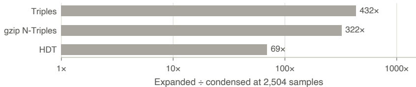
(c) Counting triples overstates the size gap
