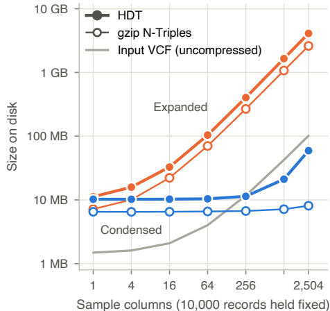
(b) Bytes: condensed still grows
