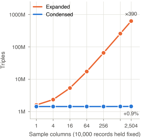
(a) Triples: condensed barely grows
