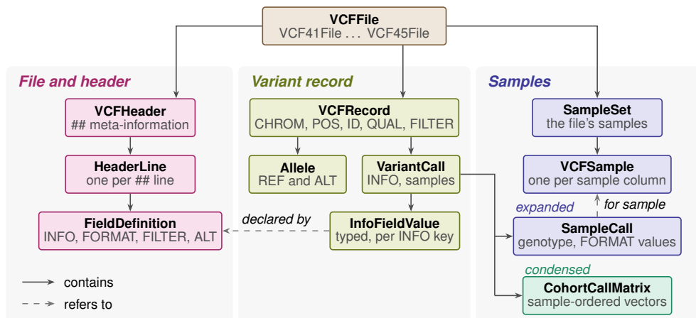
Fig. 1 Central VCF Core terms emitted by VCF-RDFizer. A versioned file contains its header, records, and sample set; a record contains alleles and a call; and the call holds INFO values and either expanded sample calls or condensed sample-ordered vectors. Values retain links to the header declarations that define them. Supplementary Figure S1 presents the fuller model.
