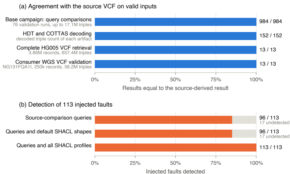
Fig. 2 Validation outcomes on valid inputs and injected faults. Panel (a) summarizes source agreement in the base campaign, native artifact decoding, and the separate complete-HG005 and consumer WGS query comparisons. Panel (b) shows detection of the 113 injected faults by source-comparison queries, the default SHACL profile, and all shape profiles.
