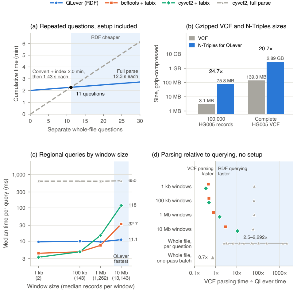
Fig. 5 VCF parsing and indexed RDF querying favor different workloads. Panel (a) includes the approximately two-minute minimal RDF setup and shows the cumulative repeated-question crossover. Panel (b) compares compressed input sizes. Panel (c) reports regional query time from 1 kb to 10 Mb. Panel (d) summarizes the ratio of VCF parsing time to QLever query time, excluding setup.
