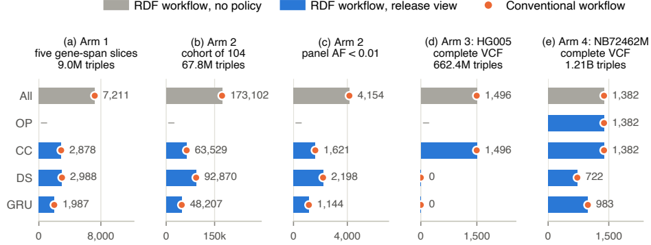
Fig. 3 The RDF and conventional workflows returned identical match sets for every requester and arm. Counts are participant–variant–gene tuples. CC denotes clinical care, DS disease-specific cardiovascular research, GRU general research use, and OP care by the participant’s physician in Arm 4. The Arm 2 rare-variant result also joins the separate panel-frequency graph at allele frequency below 0.01.
