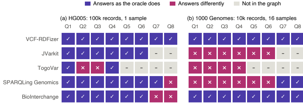
Fig. 4 Cross-vocabulary content-question results on two shared inputs. Each cell compares one ported question with the answer computed directly from the VCF: a check mark denotes agreement, a cross disagreement, and a dash information not represented in the graph. Q1–Q4 summarize records, Q5–Q6 genotypes, and Q7–Q8 the header.
