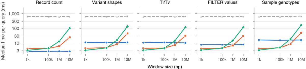
(a) Each regional question on 100,000 HG005 records (17.1M triples)
