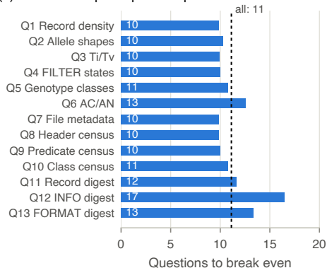
(c) Break-even per repeated question
