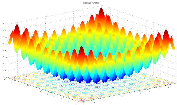
Figure 1: The Rastrigin function with the conventional A = 10 , illustrating its many local minima. The experiments below use the smoother A = 0.5 surface.
