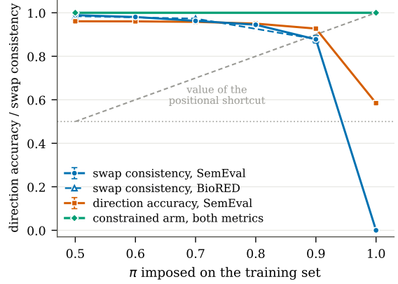
Figure 2: The same corpus at six priors. Consistency degrades while accuracy holds, until the shortcut becomes worth more than reading the passage. The constrained arm, trained on the same data, is flat at 1.000 at both extremes.
