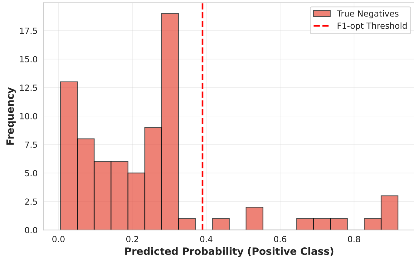
Probability Distribution (True Negative Samples)
