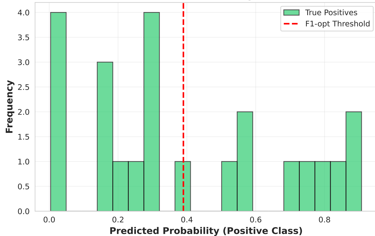
Probability Distribution (True Positive Samples)
