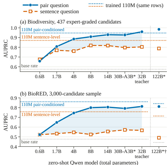
Figure 4: Zero-shot Qwen models: AUPRC of Qwen models (Qwen Team, 2025) asked the sentence question (dashed, open squares) or the pair question (solid, filled circles) on (a) the 437 expert-graded candidates and (b) a 3,000-candidate BioRED sample. Dotted: the trained 110M models on the same rows (three-checkpoint ensembles); grey: base rate. From 1.7B on, the pair question leads at each size on both benchmarks, while the sentence question gains little with scale. *Mixture of experts, placed by total size; the 32B model is the teacher. †Qwen3.5-122B-A10B (Qwen Team, 2026), a later release, ran on the first 1,000 BioRED candidates (base rate 0.442; trained models 0.714 and 0.841). Asked the triple question (our benchmark only), the models track or exceed the pair question (Appendix E).
