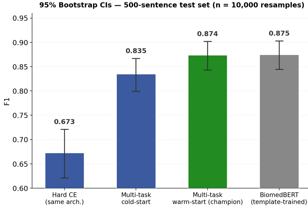
Figure 2: Bootstrap 95% confidence intervals for four models on the 500-sentence test set. Significance annotations refer to McNemar’s test.
