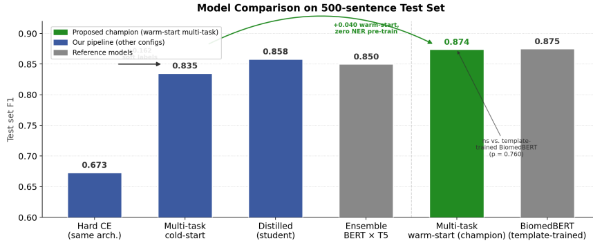
Figure E.1: Test F1 across model architecture stages (numerically in Table 2). Annotated arrows indicate the primary driver of each improvement.
