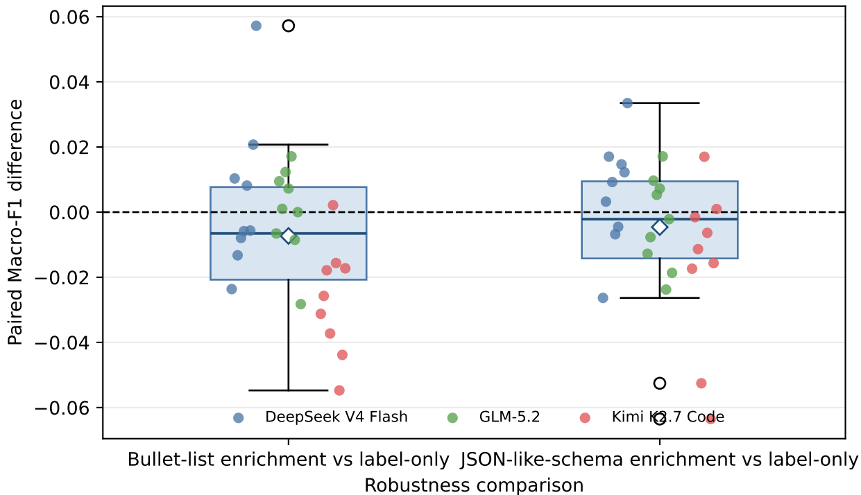
Robustness prompt effects across instructions and repeats
