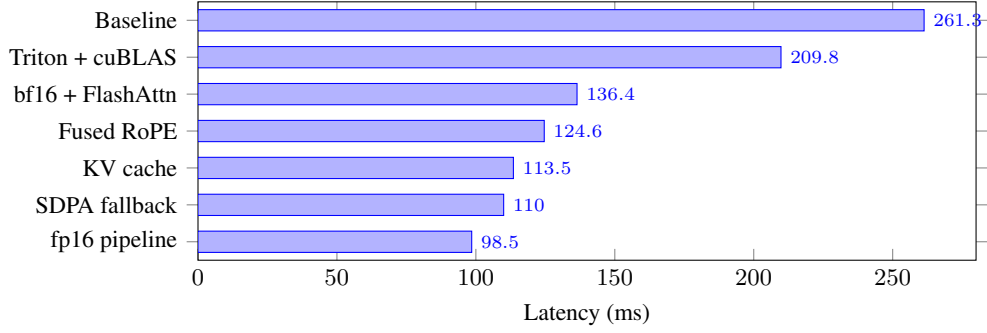
Figure 2: Optimization progression on RTX 5090 (cumulative). Each bar shows end-to-end latency after applying all optimizations up to that step. Full step-by-step breakdown in Appendix Table 8.
