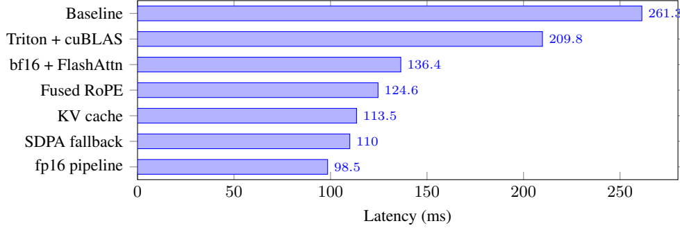
Figure 2: Optimization progression (development GPU, RTX 5090). Each bar shows end-to-end latency after applying all optimizations up to that step. Validated on H200 at 204.8 ms (Section 6). Full breakdown in Appendix Table 8.
