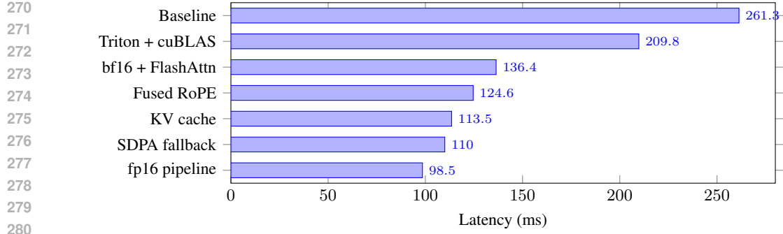
Figure 2: Optimization progression (development GPU, RTX 5090). Each bar shows end-to-end latency after applying all optimizations up to that step. Optimizations validated on H200 at 204.8 ms (Section 6). Full breakdown in Appendix Table 9.
