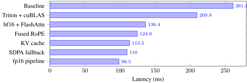
Figure 2: Optimization progression on RTX 5090 (cumulative). Each bar shows end-to-end latency after applying all optimizations up to that step. Full step-by-step breakdown in Appendix Table 9.
