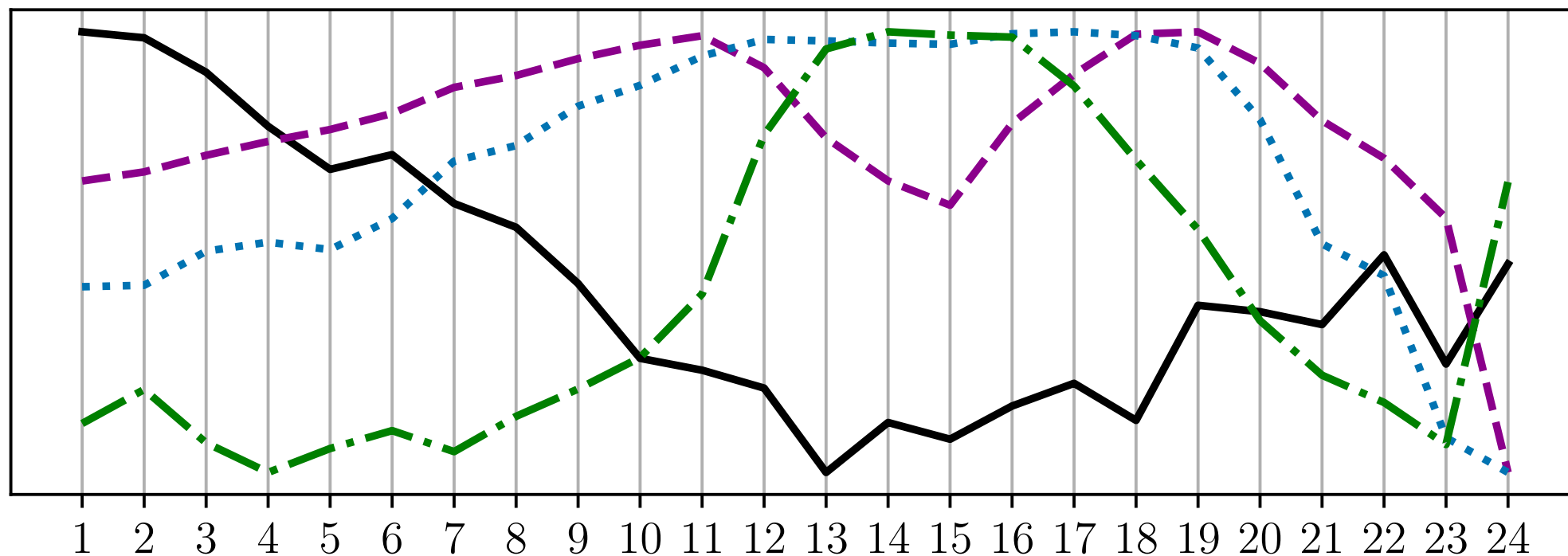
wav2vec 2.0 LARGE
