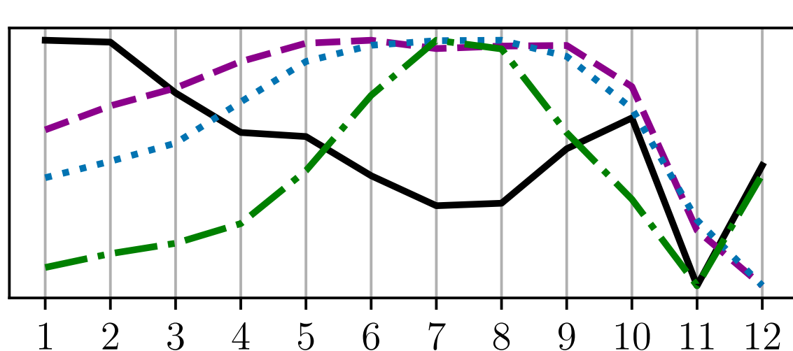
wav2vec 2.0 BASE
