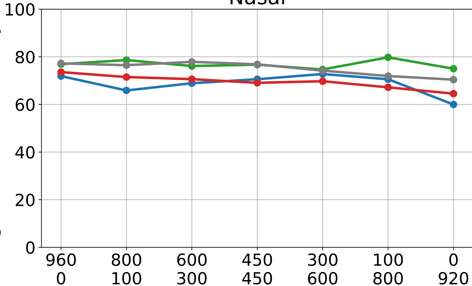
Nasal
