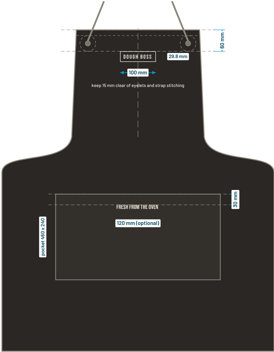
indicative outline, 900 mm long, 760 mm at the waist
