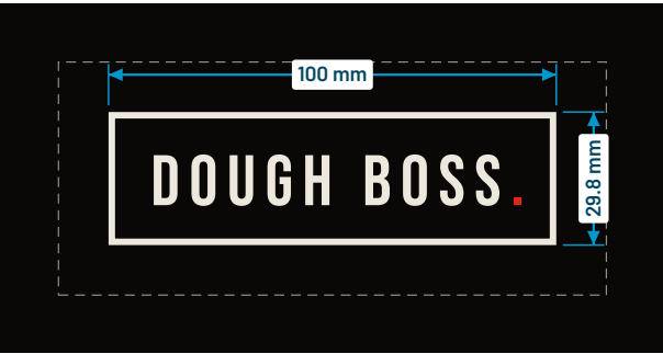
Bib wordmark, scale 1:1.9 border 1.45 mm cap height 11.2 mm type 15.97 mm clear space 11.2 mm (dashed) embroidery minimum 90 mm: PASS
