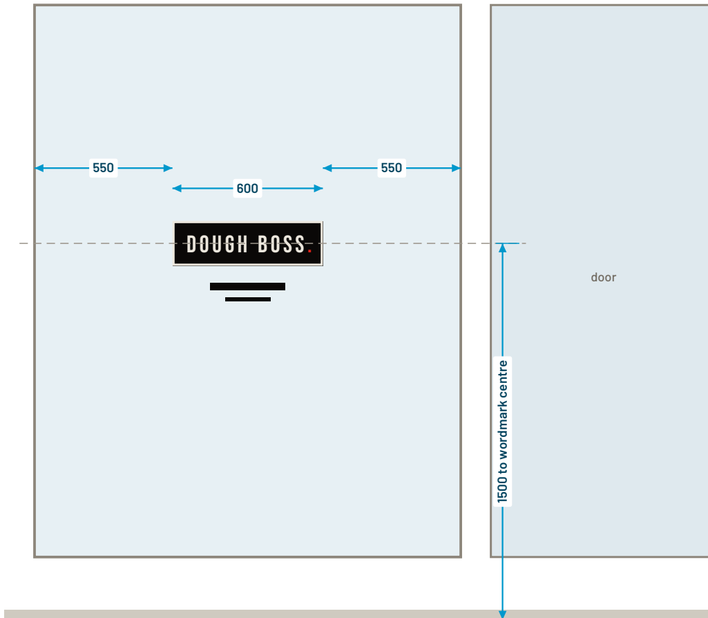
SHOPFRONT ELEVATION, seen from the street. Glazing size is illustrative [CONFIRM on site]
