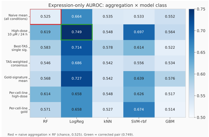
Fig. 2. Expression-only AUROC across aggregation strategies \times downstream model classes (mean over six drug classes, 6 subsampling repeats per cell). This grid shows the pattern; the four corner cells are re-estimated at 30 repeats with bootstrap intervals in Table III. Neither axis alone explains the result: the naive-aggregation/random-forest cell (red) is the weakest in the grid, while correcting both axes (green) is among the strongest. Every other cell recovers partial signal, so the suppression requires the conjunction.
