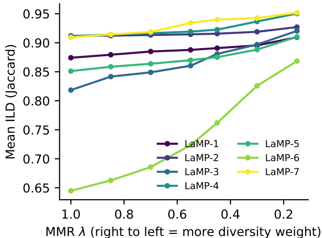
\lambda \rightarrow ILD (flan-T5-base (250M) / BM25)
