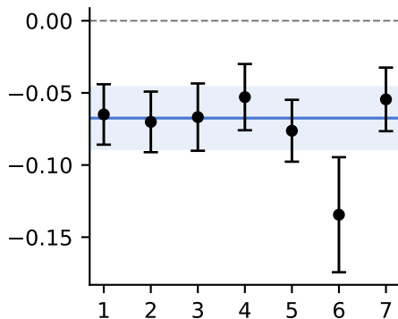
Finding 3: diversity-utility association coef( ILD_{norm} ), MMR rows only
