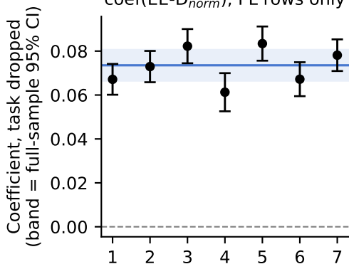
Finding 2: fairness-utility tradeoff coef( EE-D_{norm} ), PL rows only
